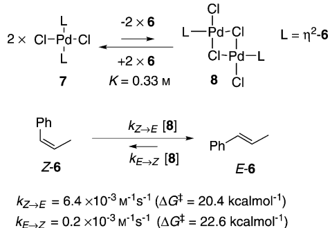
Scheme 4. Model used for simulation of the kinetics of E/Z interconversion of \beta -methyl styrene ( 6 ), starting from Z-6 (Figure 2). [12]
